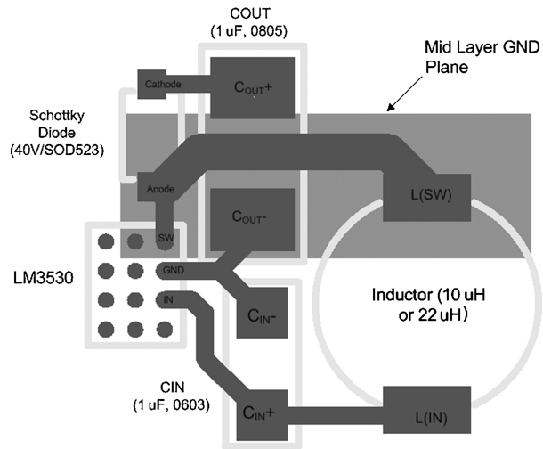
Figure 60. Layout Example #3
