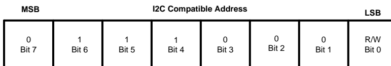
Figure 46. I 2 C-Compatible Chip Address (0x38)
