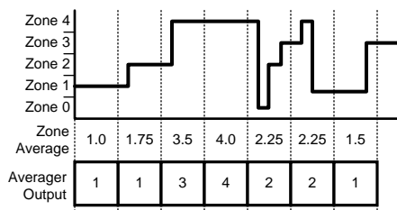
Figure 35. Averager Calculation
