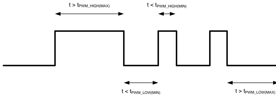
Figure 3. Simple Enable/Disable Timing
