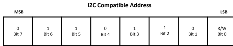
Figure 47. I 2 C-Compatible Chip Address (0x36)
