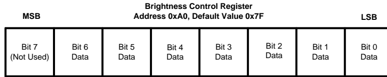
Figure 53. Brightness Control Register
