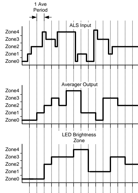
Figure 38. Perceived Brightness Change Time
