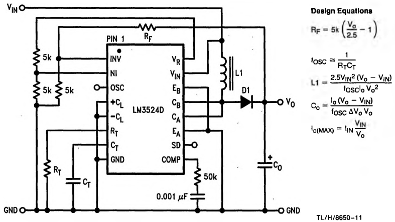
FIGURE 7. Positive Regulator, Step-Up Basic Configuration ( I_{IN(MAX)} = 80 \text{ mA} )
