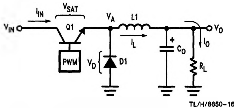
FIGURE 12. Basic Step-Down Switching Regulator
