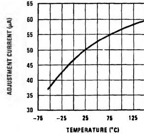
Adjustment Current
