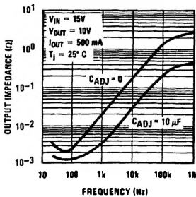
Output Impedance
