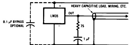
FIGURE 4. LM35 with R-C Damper
