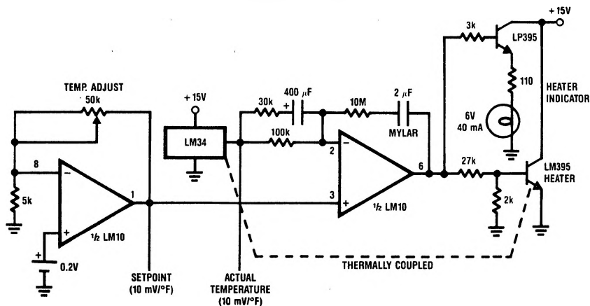
Temperature Controller
