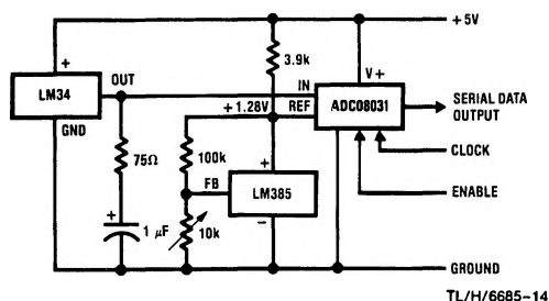
Temperature-to-Digital Converter (Serial Output, +128^{\circ}\text{F} Full Scale)
