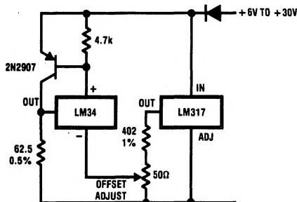
4-to-20 mA Current Source (0 to +100^{\circ}\text{F} )
