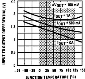
Dropout Voltage
