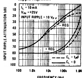
LM126 Ripple Rejection
