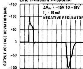
LM126 Line Transient Response
