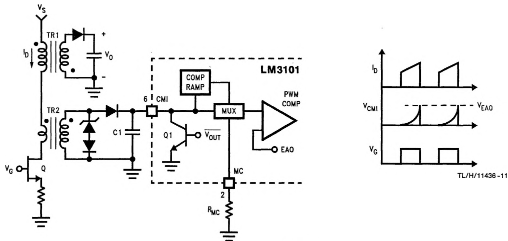
FIGURE 5. Charge Mode Operation
