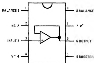
Dual-In-Line Package
