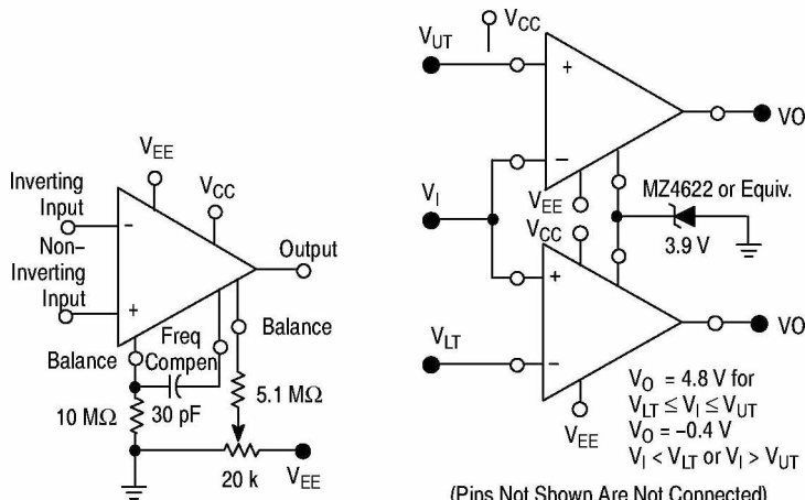
Figure 1. Standard Compensation and Offset Balancing Circuit
