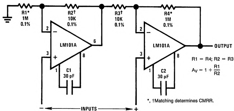
Instrumentation Amplifier
