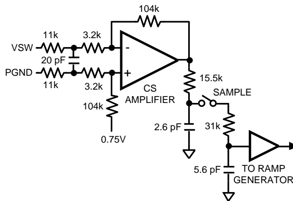
Figure 30. Current Sense Amplifier and Filter
