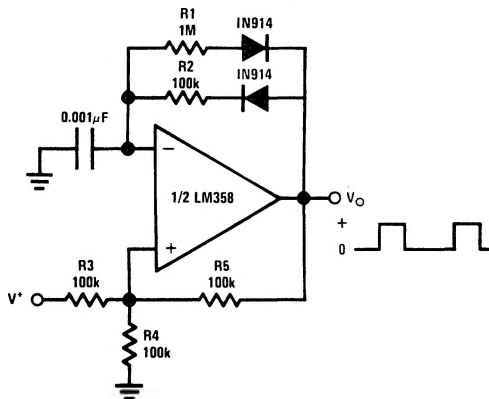
Pulse Generator
