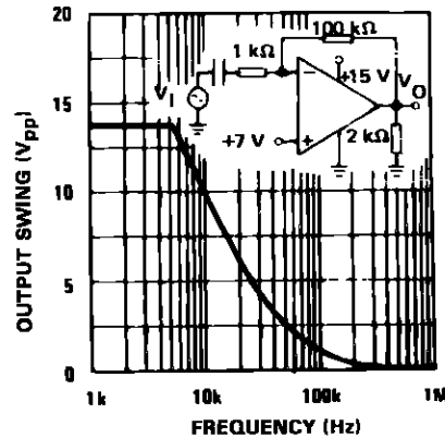
OUTPUT CHARACTERISTICS
