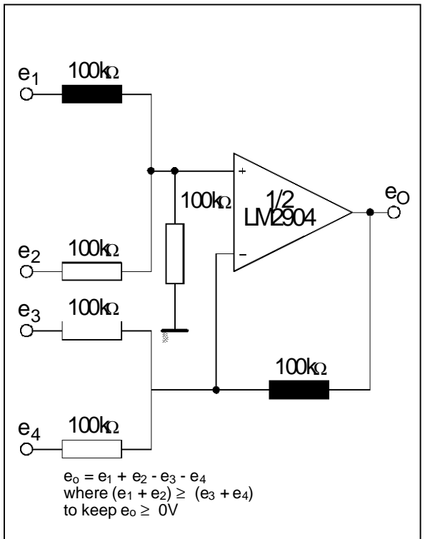
DC SUMMING AMPLIFIER
