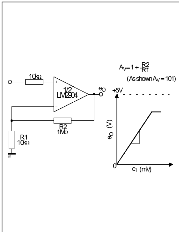
NON-INVERTING DC AMPLIFIER
