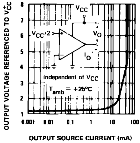
OUTPUT CHARACTERISTICS
