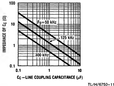
FIGURE 9. C C 's impedance should be, as a rule-of-thumb, smaller than the lowest expected line impedance
