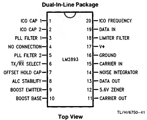
FIGURE 2. Connection Diagrams
