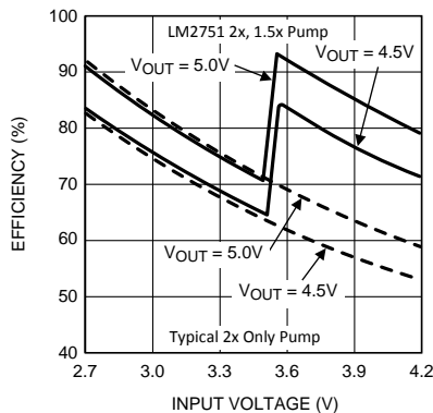
Figure 1. LM2751 2x/1.5x Efficiency vs. 2x Charge Pump Efficiency
