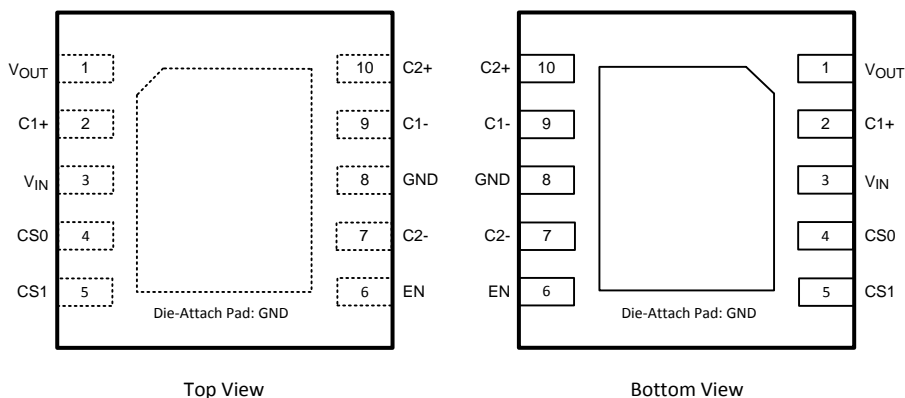
Figure 2. 10-pin SON No Pullback Package (3mm x 3mm x 0.8mm) See Package Number DSC0010A
