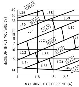
Figure 12. LM2673-12
