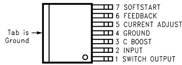
Figure 1. TO-263 Package Top View
