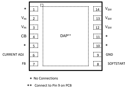
Figure 3. LLP-14 Top View
