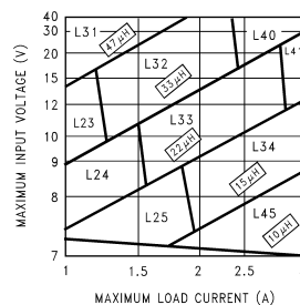
Figure 11. LM2673-5.0
