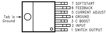
Figure 2. TO-220 Package Top View
