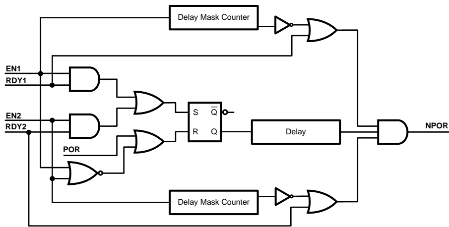
Figure 31. Design Implementation of the Flexible Power-On Reset
