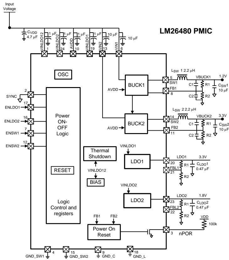
Figure 1. Application Circuit
