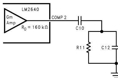
Figure 26. Typical Compensation Network
