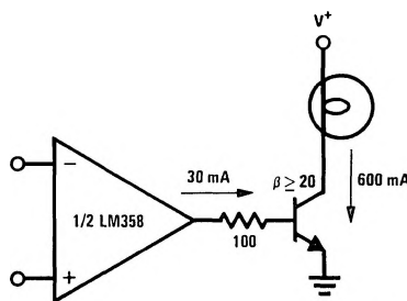
Lamp Driver
