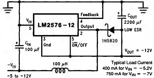
FIGURE 11. Negative Boost
