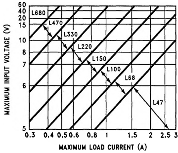
FIGURE 3. LM2576(HV)-3.3
