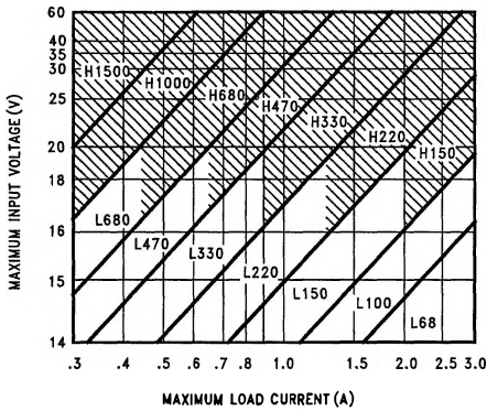
FIGURE 5. LM2576(HV)-12
