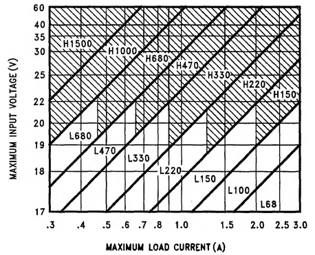
FIGURE 6. LM2576(HV)-15
