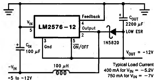
FIGURE 11. Negative Boost
