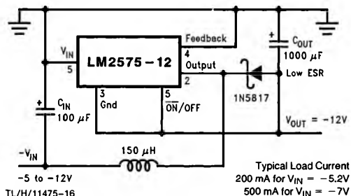
FIGURE 11. Negative Boost
