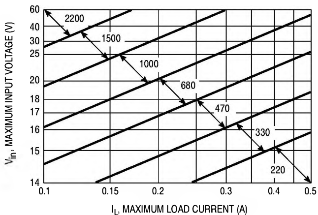
Figure 21. LM2574-12
