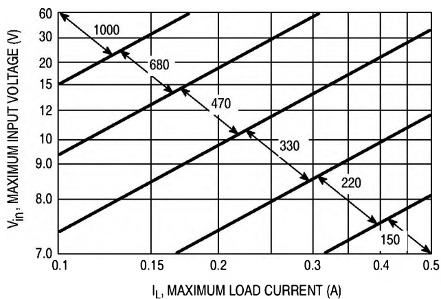
Figure 20. LM2574-5
