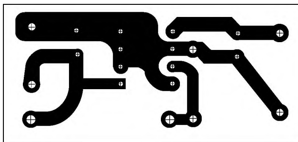
Figure 38. PC Board Layout Copper Side
