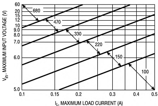
Figure 19. LM2574-3.3
