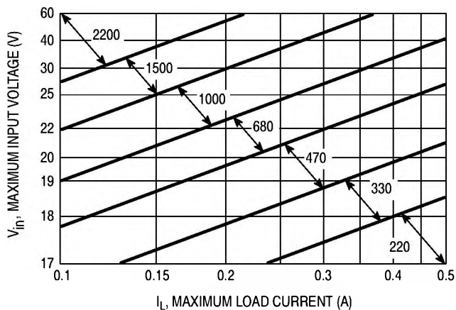
Figure 22. LM2574-15
