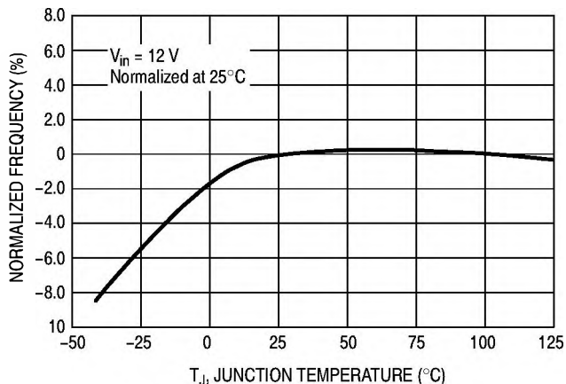
Figure 8. Oscillator Frequency
