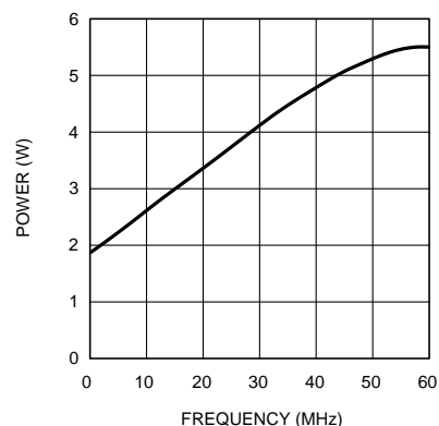
Figure 7. Power Dissipation vs Frequency
