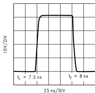
Figure 6. LM2466 Pulse Response
