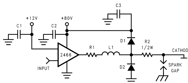
Figure 10. One Channel of the LM2466 with the Recommended Application Circuit
