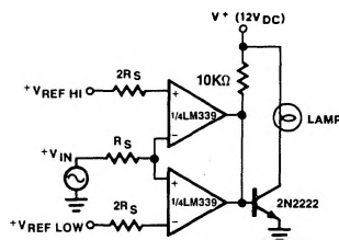
LIMIT COMPARATOR
