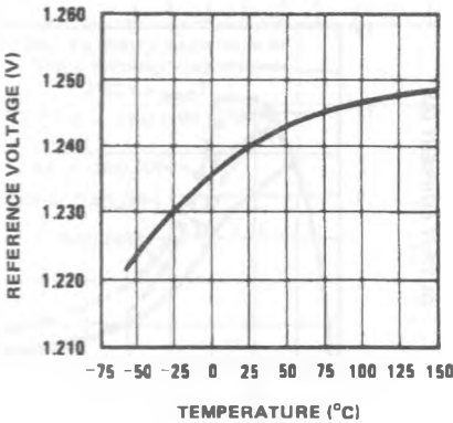
TEMPERATURE STABILITY
