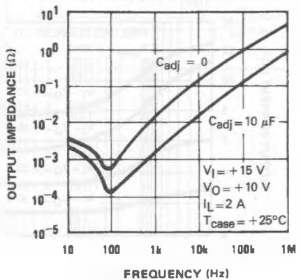
OUTPUT IMPEDANCE
