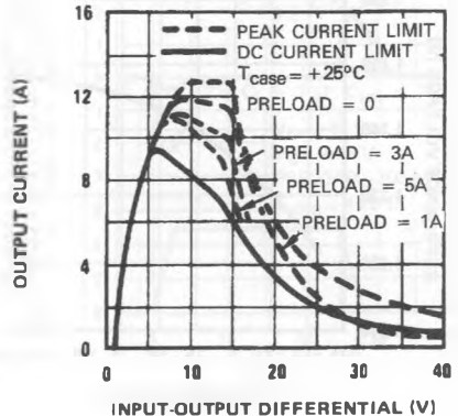
CURRENT LIMIT
