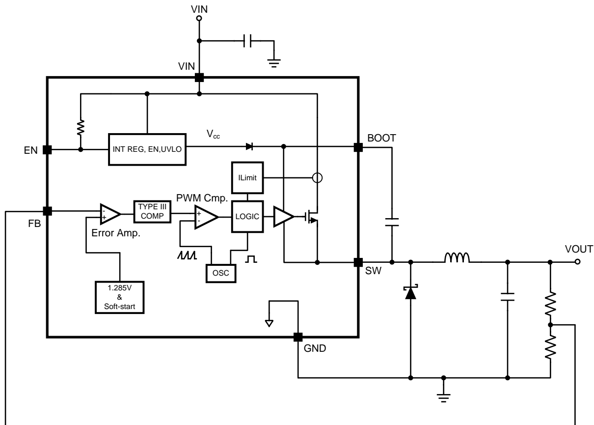
Figure 11. Simplified Block Diagram
