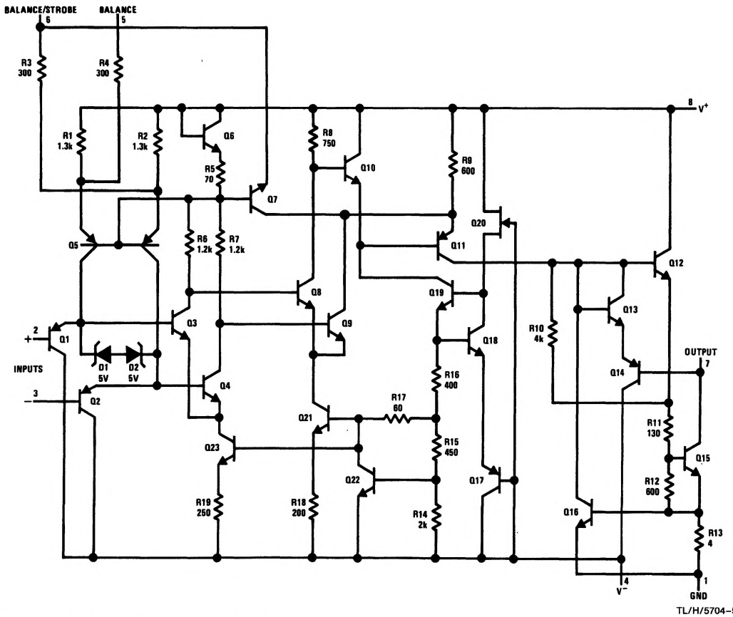
TL/H/5704-5
