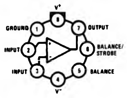
TL/H/5704-6
