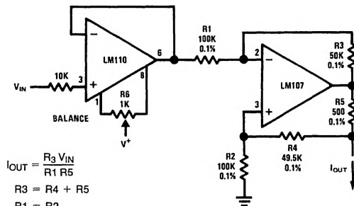
Bilateral Current Source
