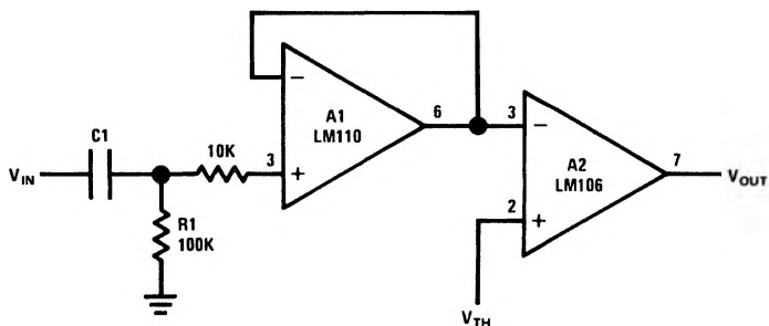
Comparator for AC Coupled Signals
