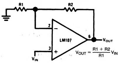
Non-Inverting Amplifier
