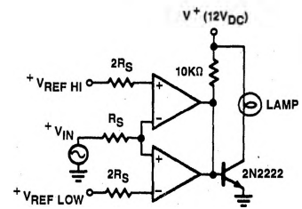
LIMIT COMPARATOR
