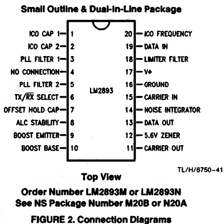
FIGURE 2. Connection Diagrams
