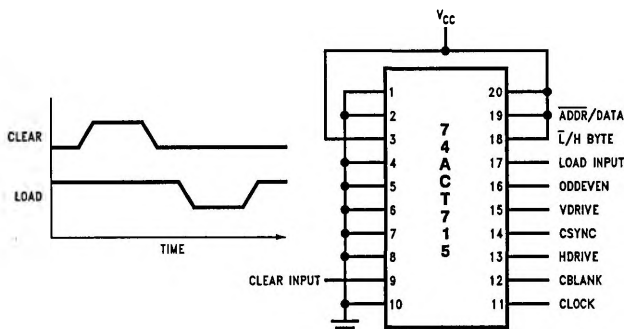
FIGURE 5. Default RS170 Hardwire Configuration
