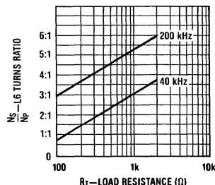
FIGURE 6. L6 Turns Ratio vs Load Resistance
