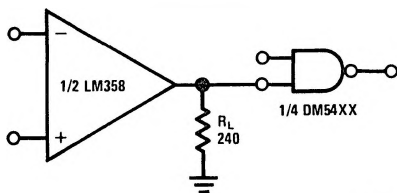
Driving TTL
