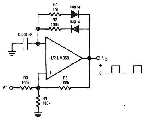
Pulse Generator
