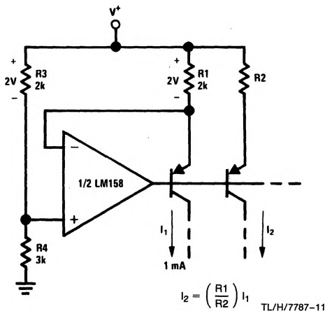
LED Driver
