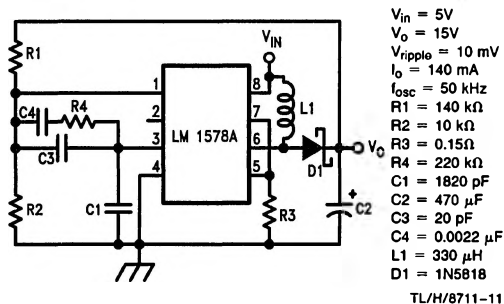
FIGURE 19. Boost or Step-Up Regulator
