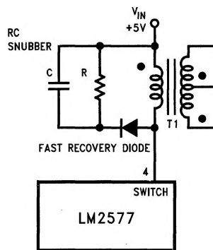
FIGURE 19. Snubber Circuit
