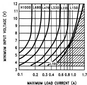
FIGURE 7b. LM2577-15 Inductor Selection Guide
