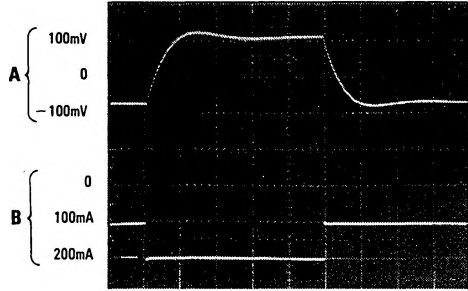
FIGURE 24. Load Transient Response of Flyback Regulator of Figure 20, -15V Output
