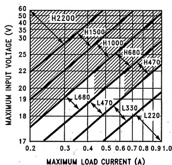
FIGURE 6. LM2575(HV)-15
