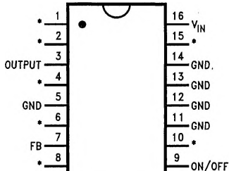
16-Lead DIP (N)
