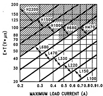
FIGURE 7. LM2575(HV)-ADJ
