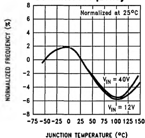
Oscillator Frequency
