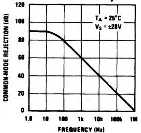
Common-Mode Rejection
