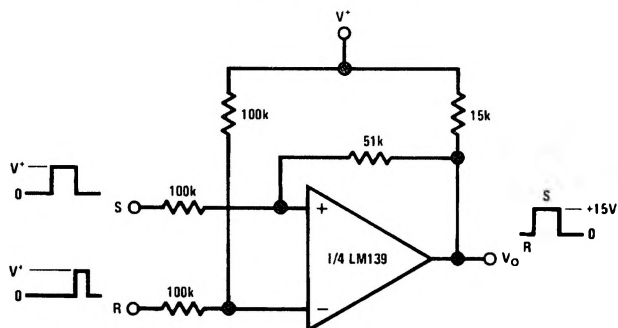
Bi-Stable Multivibrator
