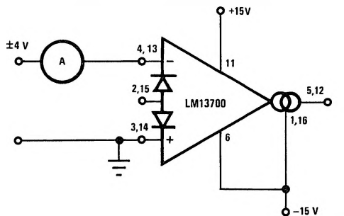
Differential Input Current Test Circuit
