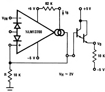
FIGURE 22. Schmitt Trigger
