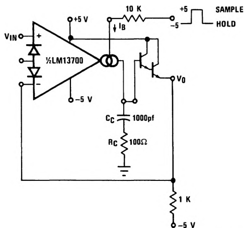
FIGURE 25. Sample-Hold Circuit
