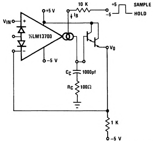
FIGURE 25. Sample-Hold Circuit
