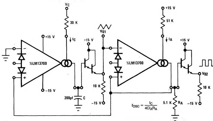
FIGURE 15. Triangular/Square-Wave VCO
