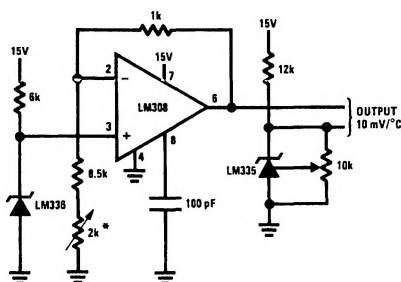
Centigrade Thermometer
