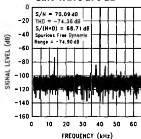
Bipolar Spectral Response with 62.25 kHz Sine Wave at 0 dB
