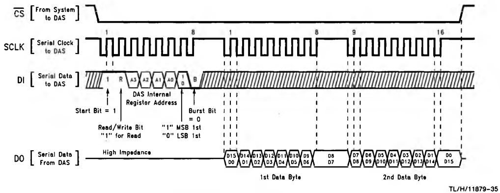
(f) Read Cycle, R/F Input (P1) = 1
