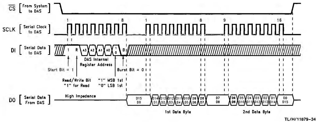
(e) Read Cycle, R/F Input (P1) = 1
