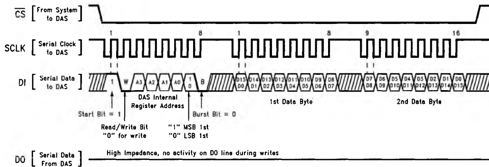
FIGURE 11. Timing Diagrams for LM12434 and LM12(L)438 Standard Serial Interface
