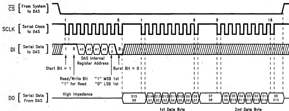
FIGURE 11. Timing Diagrams for LM12434 and LM12(L)438 Standard Serial Interface (Continued)
