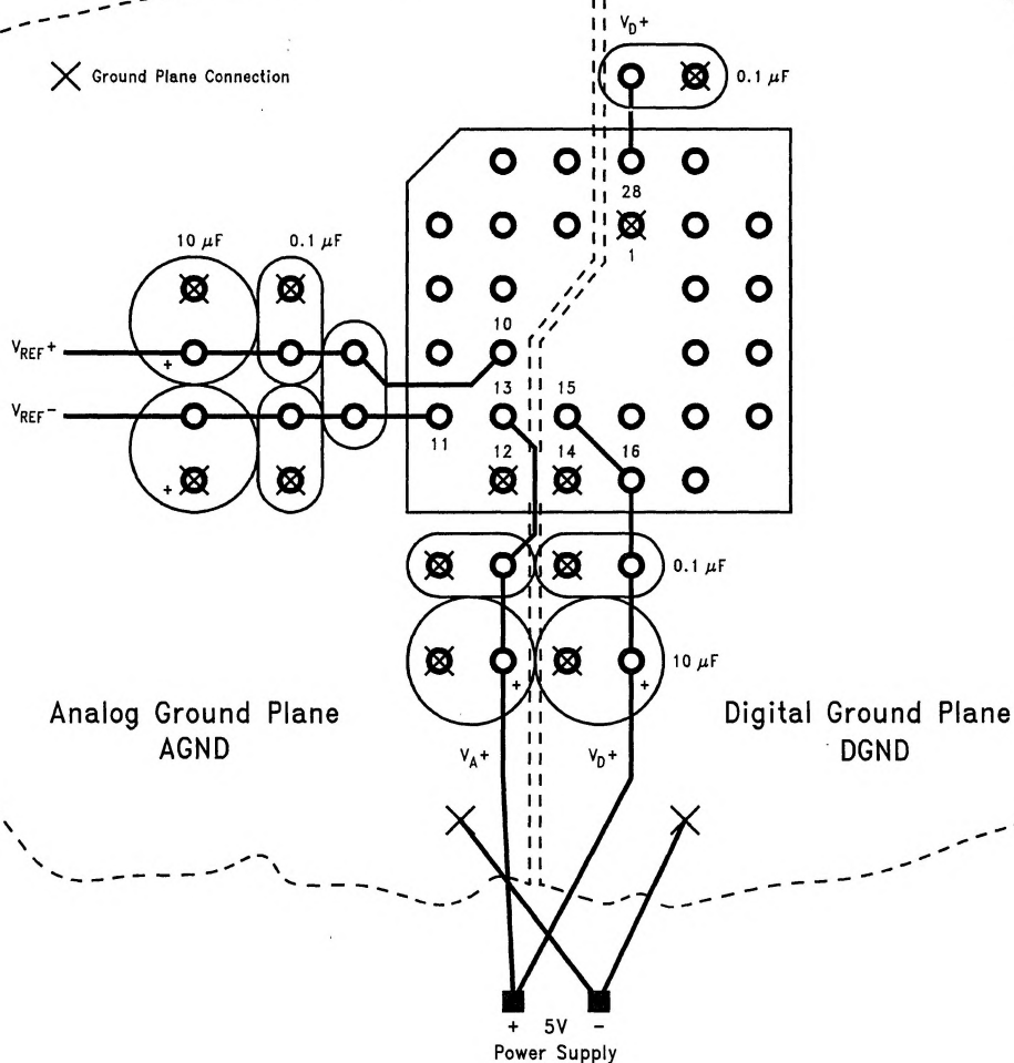
(a) Through Hole Technology with 28-Pin PLCC Socket
