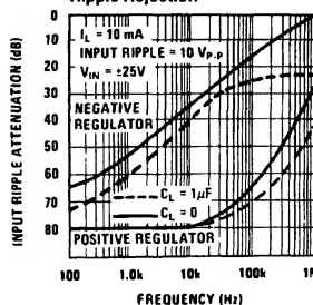
LM125 Ripple Rejection
