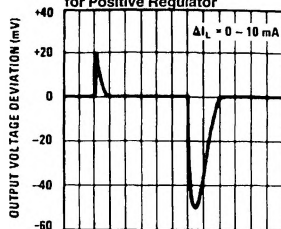
LM125 Load Transient Response for Positive Regulator
